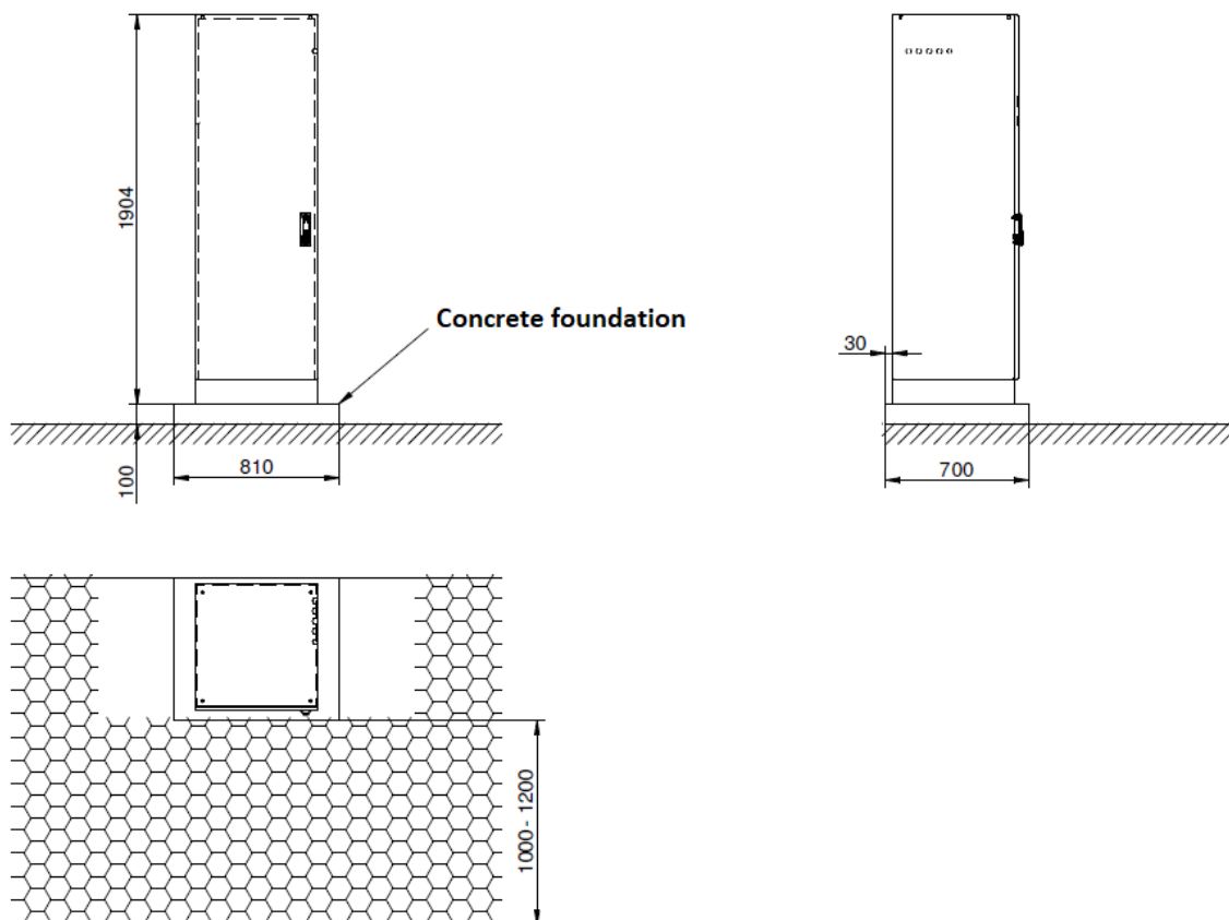
Dimensional sketch:
